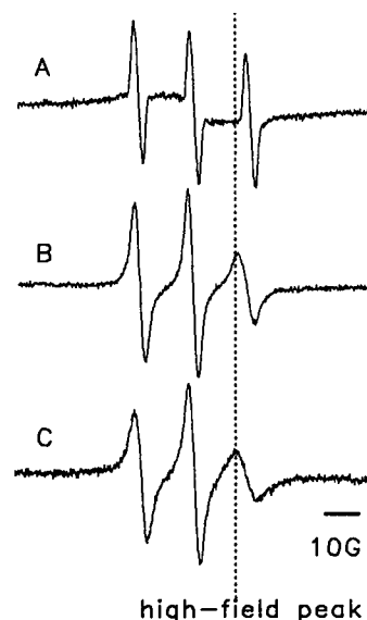
FIGURE 2 Incorporation of SL-PC into EPC vesicle membranes and red cell ghost membranes. The top spectrum (A) is the spectrum of SL-PC in aqueous buffer. Spectrum B was recorded after quantitative incorporation of SL-PC into EPC vesicle membranes (molar ratio SL-PC:EPC = 5:100). Spectrum C was recorded after incorporation of SL-PC into red cell ghost membranes (molar ratio SL-PC to ghost phospholipids = 5:100). All spectra were recorded at room temperature. The specific parameters of EPR measurement were: conversion time, 81.92 ms (A, B), 163.64 ms (C); time constant, 20.48 ms (A, B), 40.96 ms (C).
