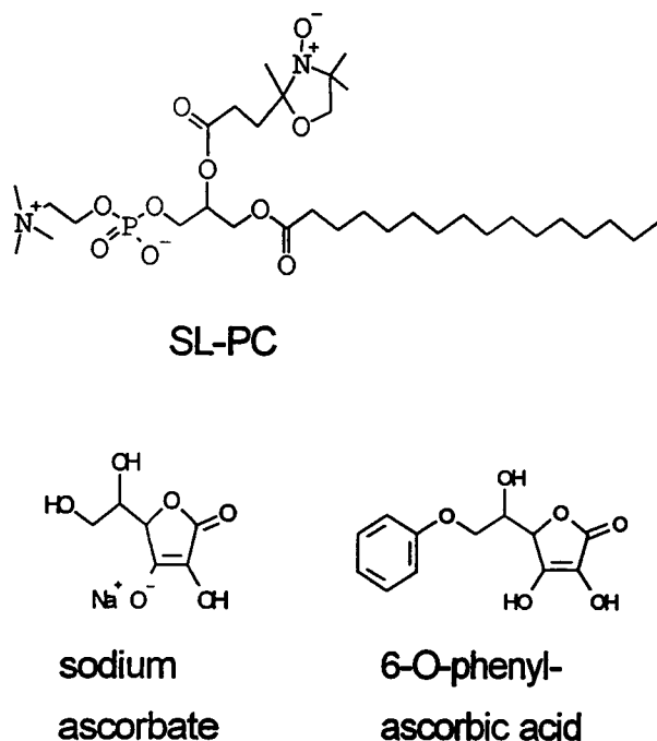
FIGURE 1 Structures of 1-palmitoyl-2-(4-doxylpentanoyl)-phosphatidylcholine, sodium ascorbate, and of 6-O-phenyl-ascorbic acid.
